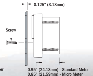
Panel Mount
